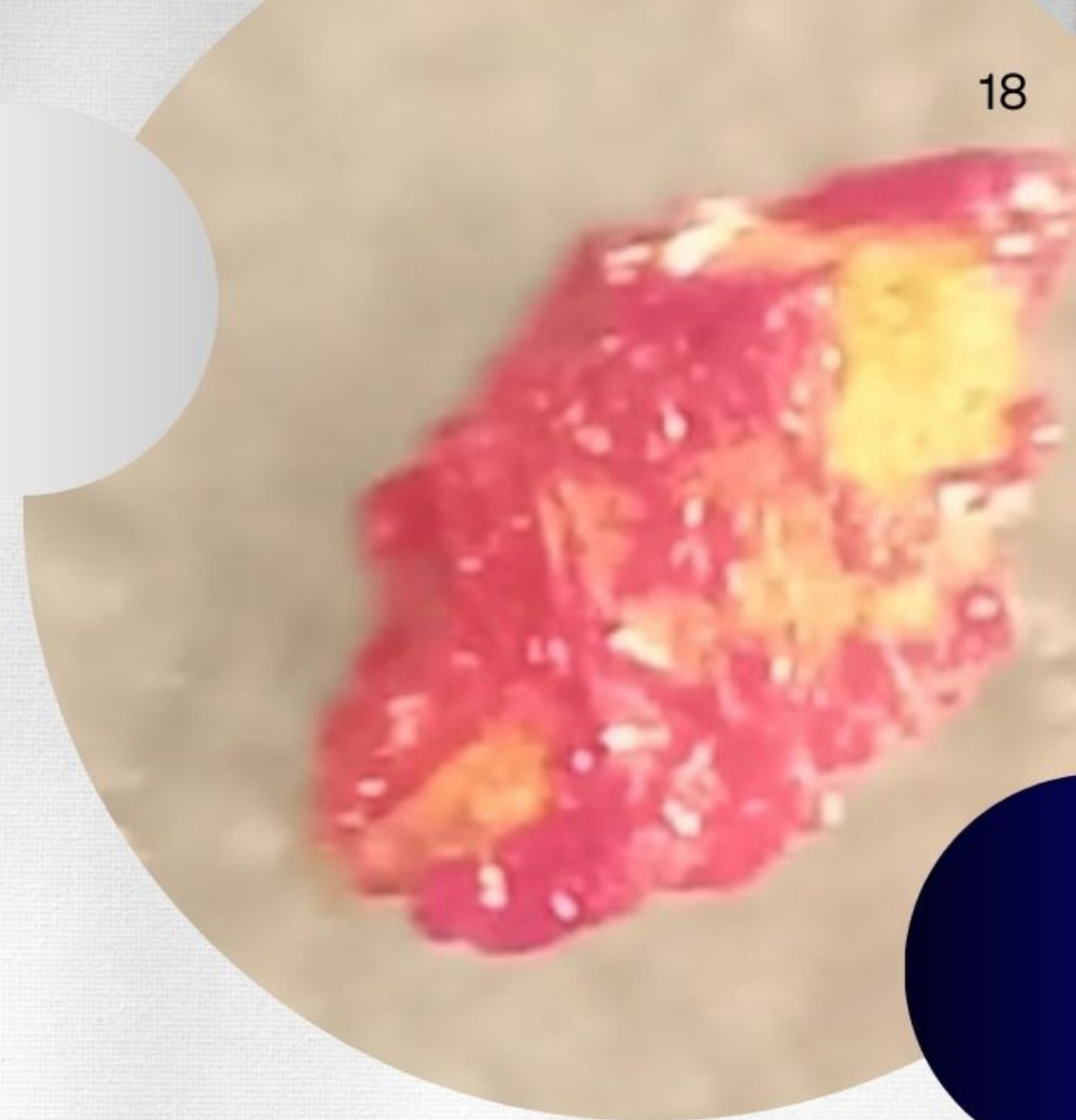
Cinnabar ~ 250 microns across
