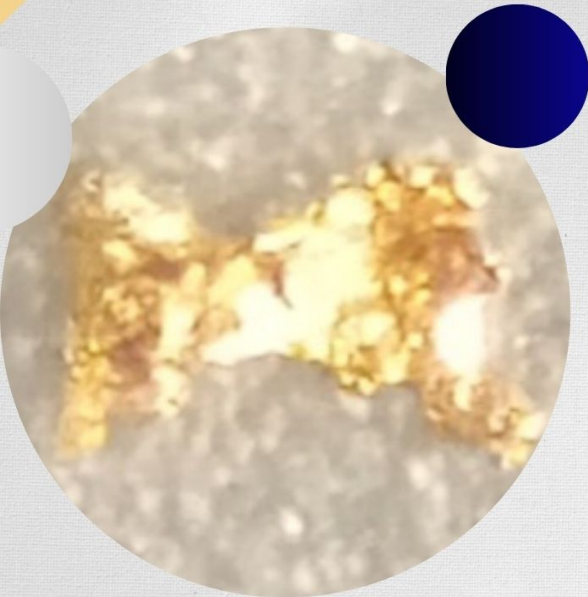
Gold Grain ~ 150 microns across
